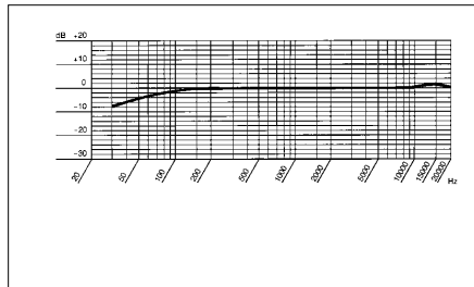
Frequenzgang
